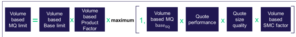
Equation 4 : Calculation of the minimum quotation limit for the volume based Order to Trade Ratio
