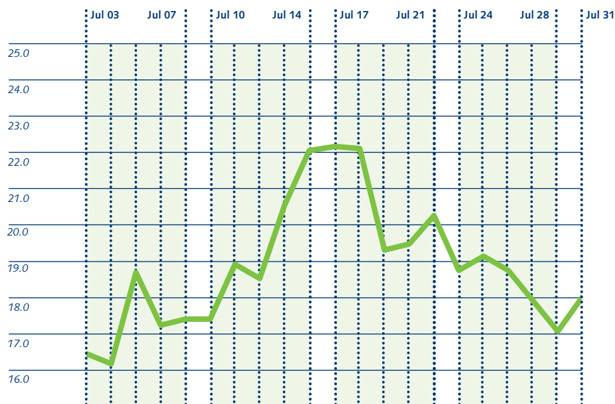
VDAX (in Percent, at Day End): July 2006
