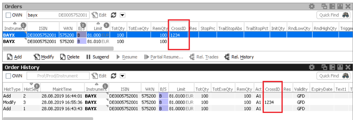
Fig. 61: Screenshots showing the CrossID column of the Orders and Order History view
