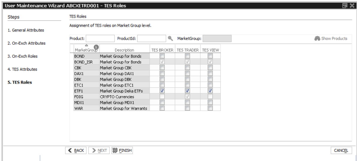
Fig. 99: Screenshot of the User Maintenance Wizard showing the TES roles tab
