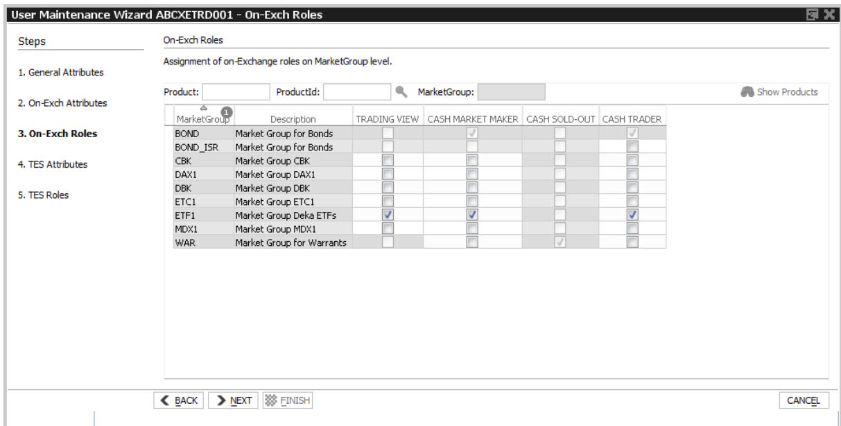
Fig. 101: Screenshot of the User Maintenance Wizard showing the entitlement roles on the On-Exch Roles tab
